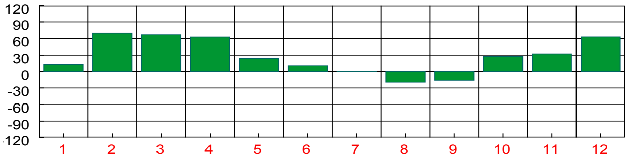
Bhavadrishi Bala
