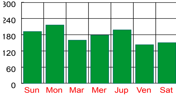
Kala Bala
