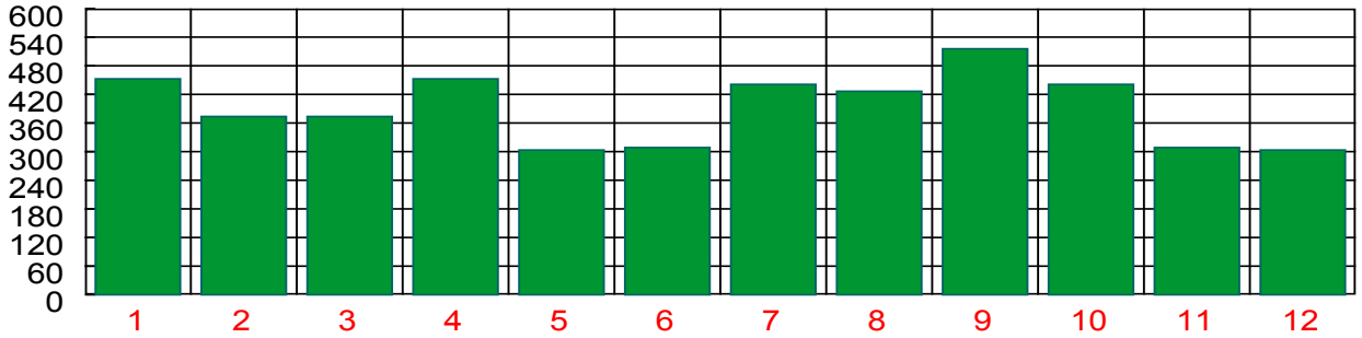
Bhavadipati Bala
