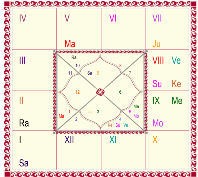
Cusp Chart
