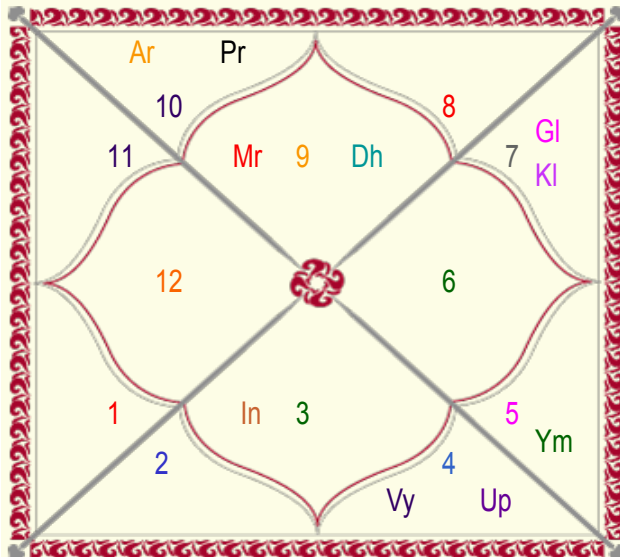
Upagraha Chart
