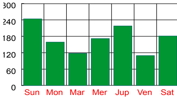
Naisargeka Bala
