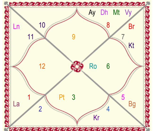
Arudha Chart
