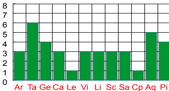
Saturn
