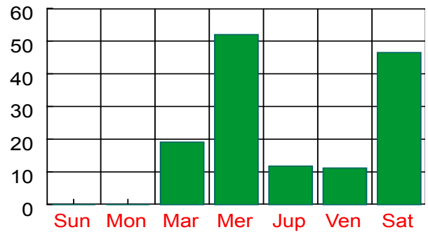
Drik Bala
