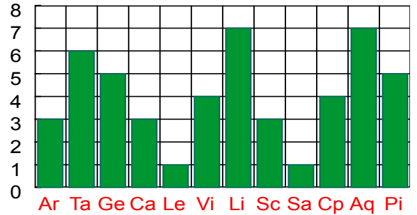
Mercury
