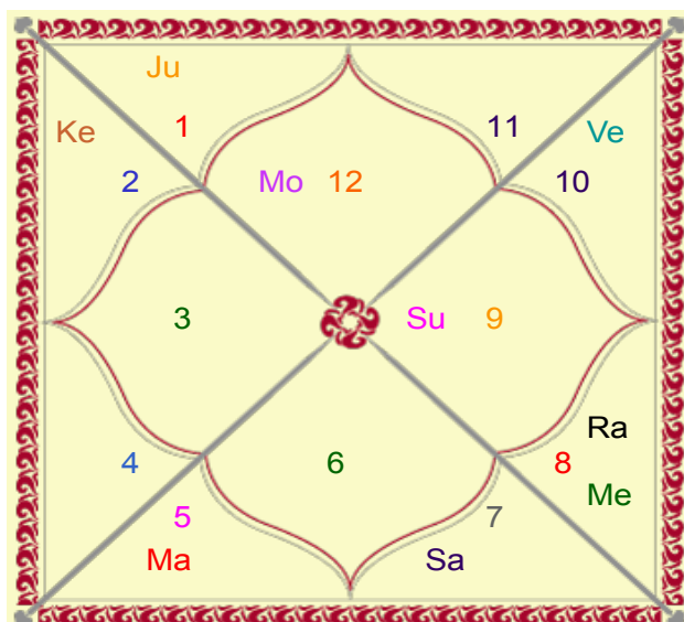
Moon Chart
