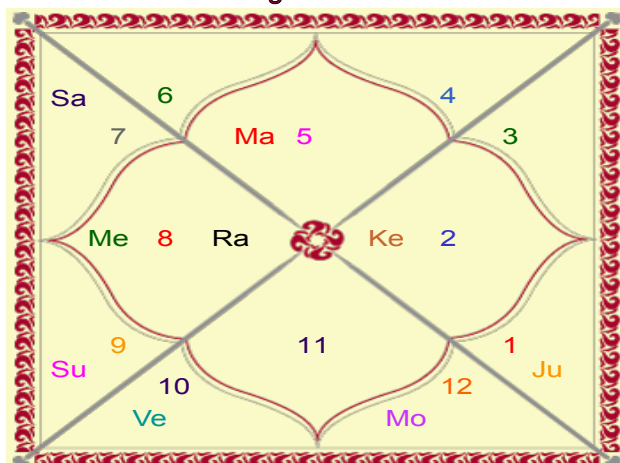
Lagna Chart
